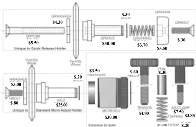
SCHRIBER QUICK CHANGE STYLE HOLDER
